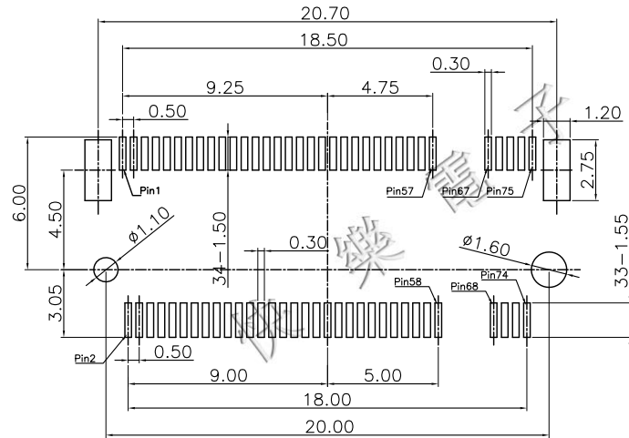
Recommended PCB Layout (Top View) Default Tolerance ±0.05
